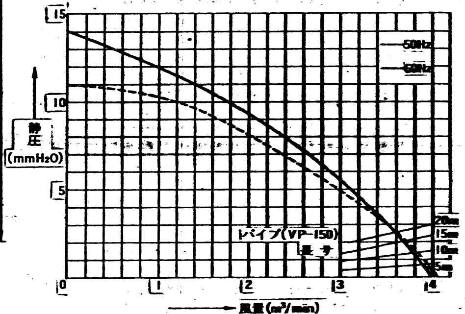
●静圧-風量特性(DVF-18XM)
