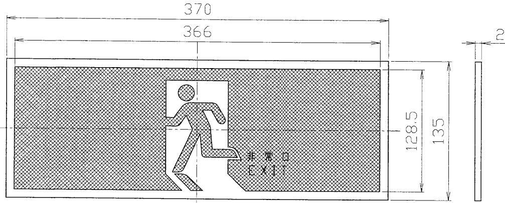
ET-1030Z
