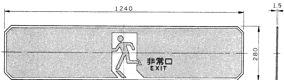
ET-4010N
