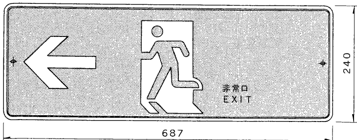
ET-2042
